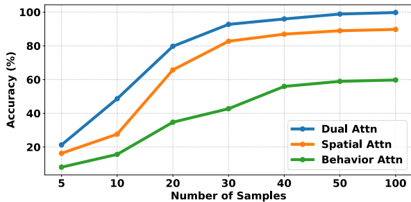
Fig. 3. Effectiveness of the Dual-Encoder
