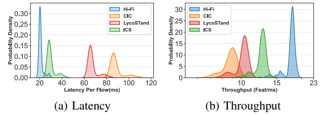
Fig. 5. Performance Overhead Evaluation
