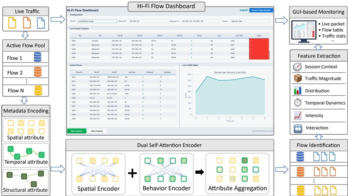
Fig. 1. System Overview of Hi-Fi Flow
